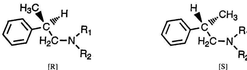
Figure 2. 3a ( R_1 = R_2 = H ) 4a ( R_1 = CH_3 ; R_2 = H ) 5a ( R_1 = CH_3 ; R_2 = CH_2C\equiv CH )
