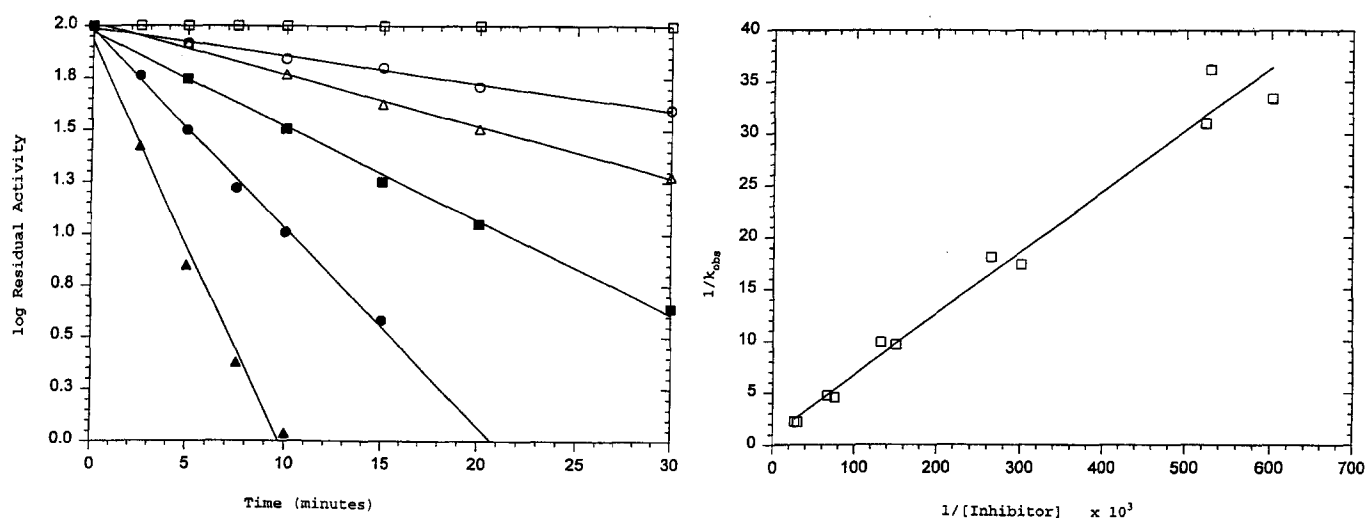
Figure 4. a. Time-dependent inhibition of MAO-B by [R]-(-)-N-methyl-N-propargyl-2-phenylpropylamine hydrochloride ( 5a ) (typical data from one experiment). Plot of log (% residual activity) against incubation time. All points are the mean of duplicate determinations. Concentrations of 5a are 0 μM (□); 1.66 μM (○); 3.32 μM (△); 6.64 μM (■); 13.29 μM (●); 33.22 μM (▲). b. Plot of 1/k_{\text{obs}} (data from figure 4a plus additional experiments) against 1/[I] . The line is that of best fit by linear regression.
