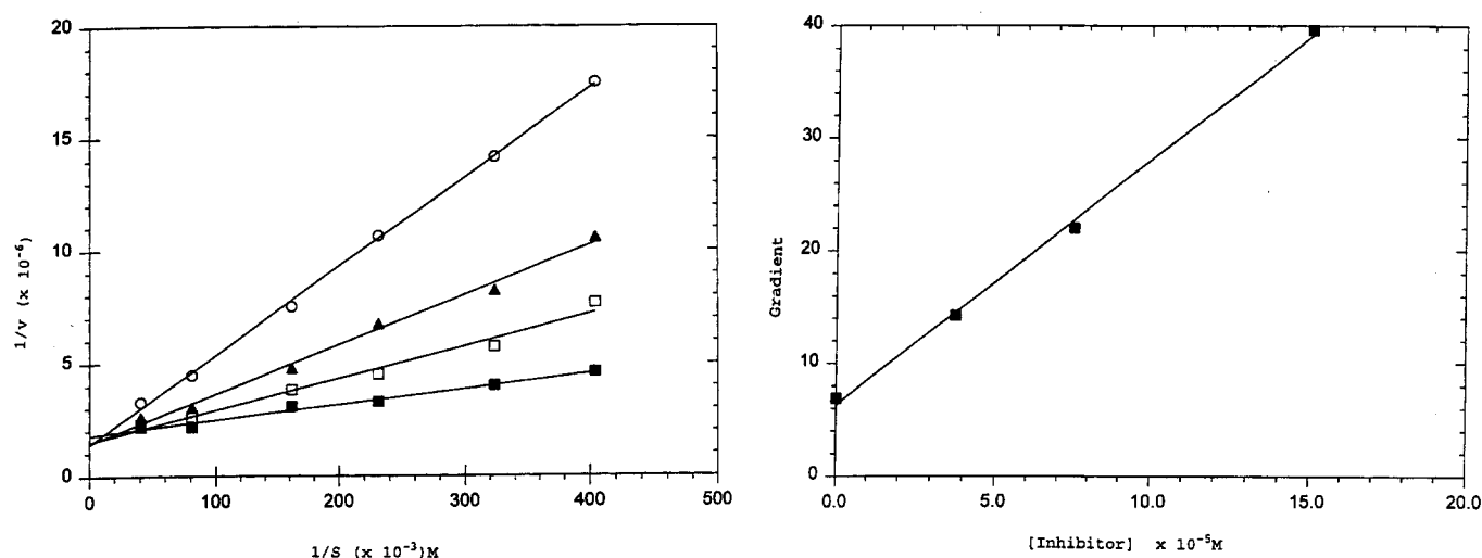
Figure 3. a. Double-reciprocal plot of inhibition of oxidative deamination of PEA by [R]-(-)-N-methyl-N-propargyl-2-phenylpropylamine hydrochloride ( 5a ). All points are the mean of duplicate determinations. Inhibitor concentrations are 0 \mu\text{M} (■); 37.66 \mu\text{M} (□); 75.32 \mu\text{M} (▲); 150.6 \mu\text{M} (○). b. Replot of gradient vs. inhibitor concentration, data from figure 3a.
