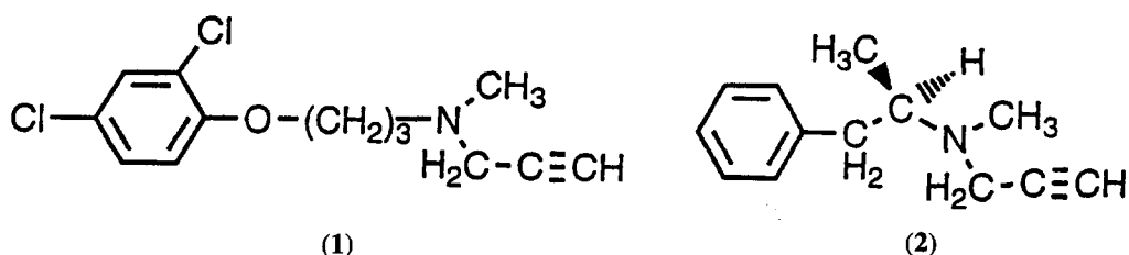
Figure 1. Structures of compounds 1 and 2 .
